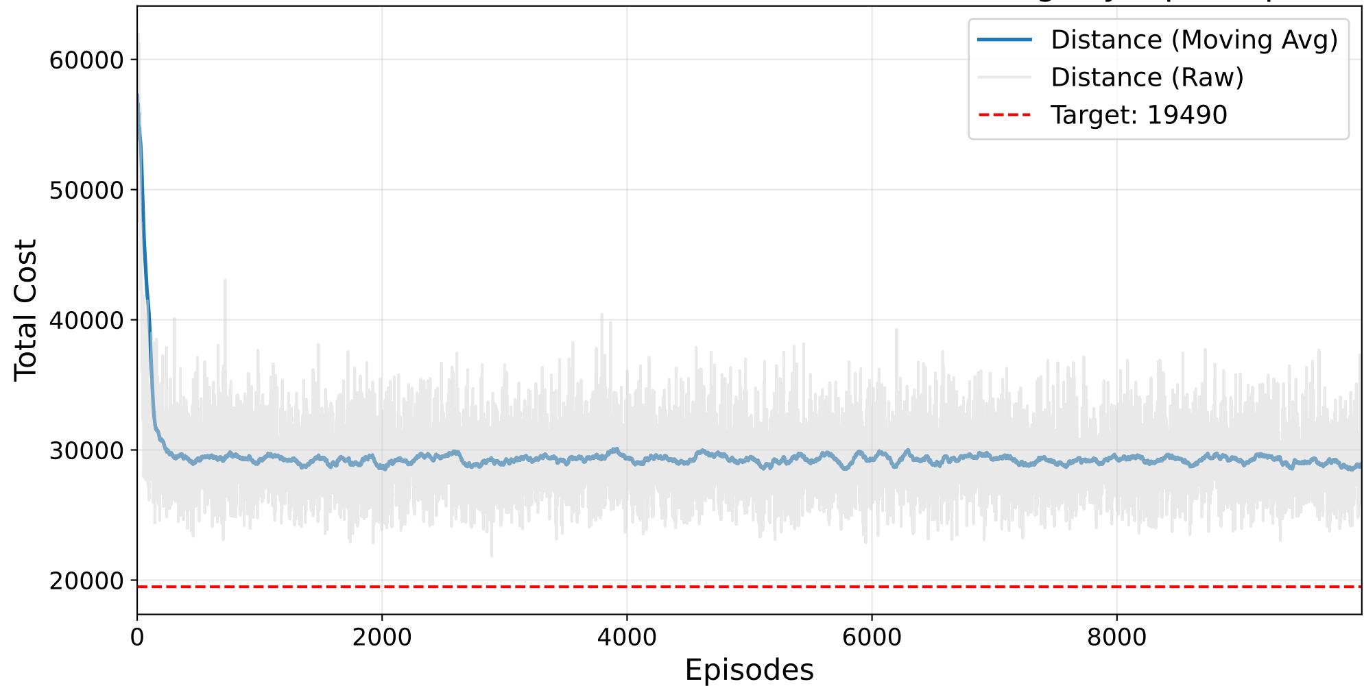
Final HYPERBAND TPE Masked AutoRL-SOP Training - ry48p.3.sop
